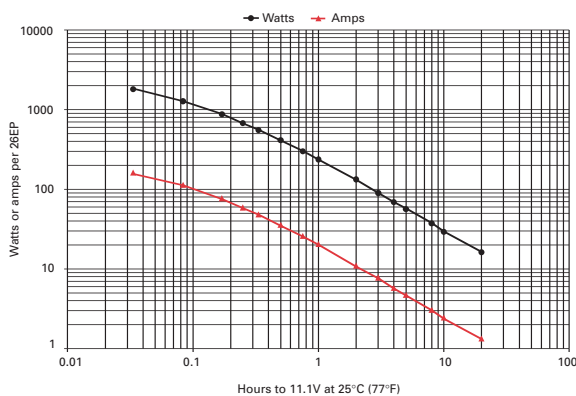
Figure B-12: 26EP discharge data to 11.1V at 25°C (77°F)
